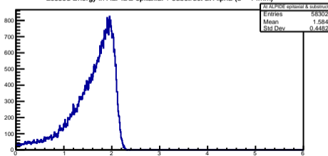
Lossed Energy in ALPIDE epitaxial + substruct at Alpha (d = 14mm)
