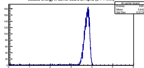
Lossed Energy in carrier board at Alpha (d = 14mm)
