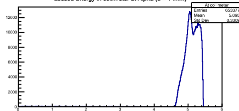
Lossed Energy in collimeter at Alpha (d = 14mm)
