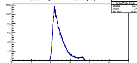
Lossed Energy in ALPIDE circuit at Alpha (d = 14mm)
