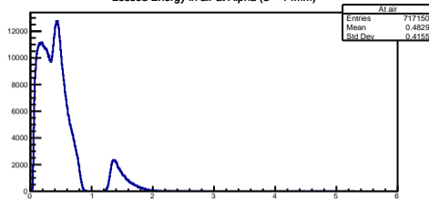
Lossed Energy in air at Alpha (d = 14mm)
